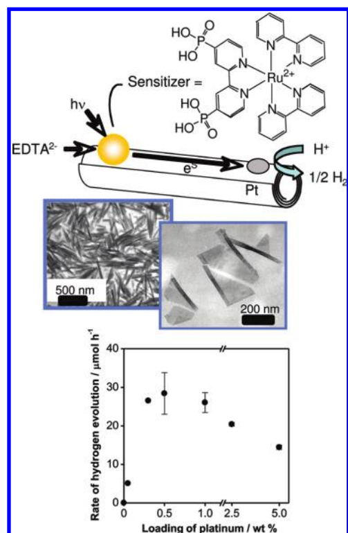
FIGURE 4. (top) Schematic representation of photoinduced electron transfer from a phosphonated [\text{Ru}(\text{bpy})_3]^{2+} sensitizer to Pt catalyst particles, mediated by LMOS nanoscrolls derived from \text{H}_4\text{Nb}_6\text{O}_{17} . (center) TEM images of the scrolling of individual nanosheets (right) and of nanoscrolls precipitated from a suspension of exfoliated \text{H}_4\text{Nb}_6\text{O}_{17} (left). (bottom) The dependence of the rate of hydrogen evolution on Pt loading and the high quantum yield establish that electron transfer from \text{EDTA}^{2-} to \text{Ru}^{3+} is the slowest step in the overall process.
