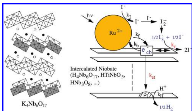
FIGURE 3. Scheme for visible light evolution from aqueous I^- , a nonsacrificial electron donor. Electron transfer to the hydrogen-evolving Pt catalyst ( k_{et} ) occurs on a time scale of tens of milliseconds. The idealized structure of the LMOS K_4Nb_6O_{17} is shown at the left.
